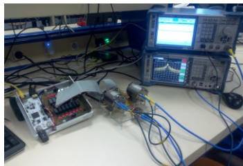
Fig. 11. Real vision of the RF device characterisation remote laboratory
