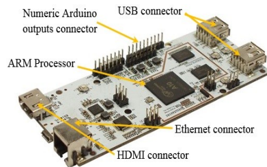
Fig. 5. First release of PCDuino platform
