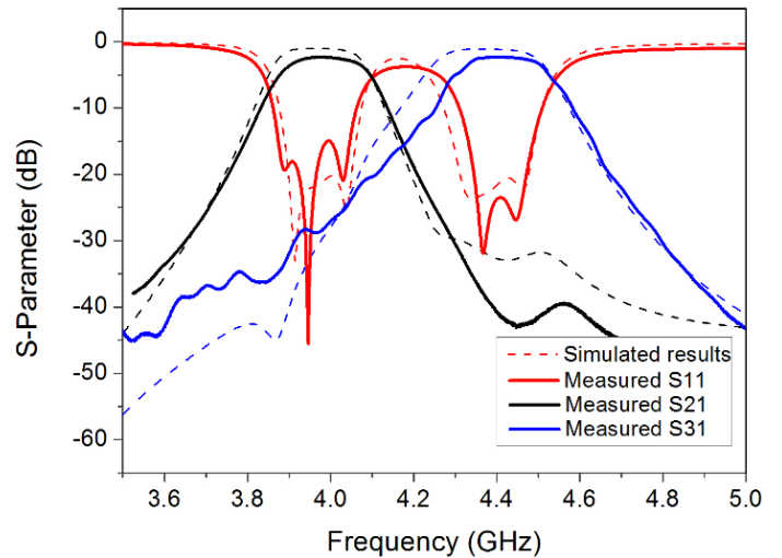
Fig. 7. Measured responses in comparison with full-wave simulations.
