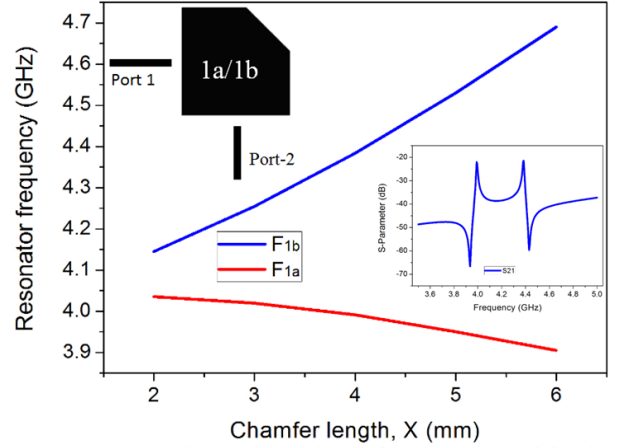
Fig. 3. Two resonance frequencies of the patch as a function of the chamfer length. The insets shows the layout used in the simulation and a typical simulated S_{21} response.
