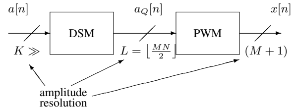
Fig. 4. Block diagram of the proposed DSM-PWM architecture.
