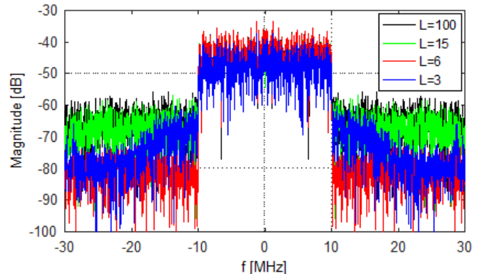
Fig. 5. Baseband spectrum of DSM-PWM output for various selection of DSM quantization levels.
