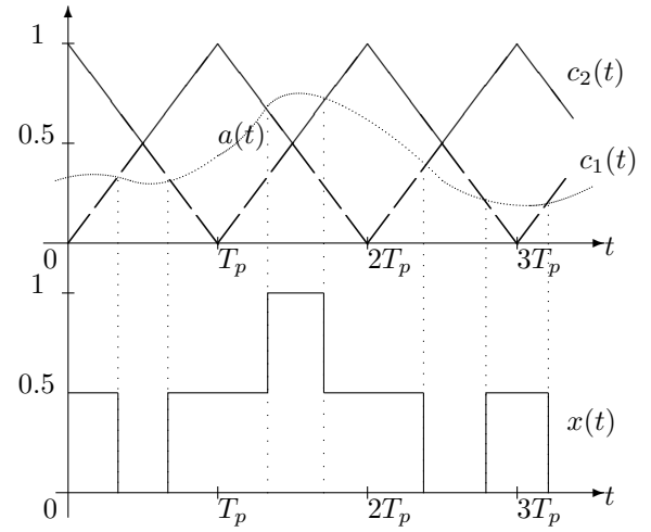
Fig. 3. PWM basic operation.
