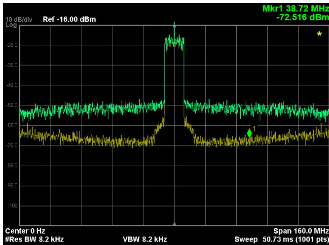
Fig. 6. Measured baseband spectrum of the PWM (green) and DSM-PWM (yellow) outputs.
