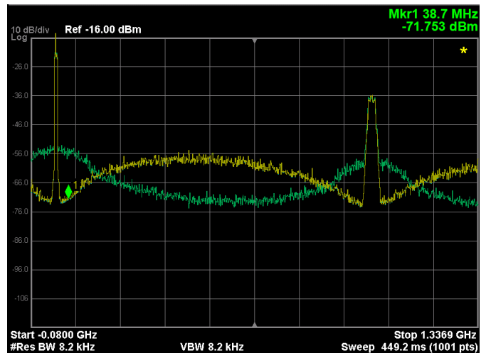
Fig. 7. Measured wideband spectrum of the PWM (green) and DSM-PWM (yellow) outputs.
