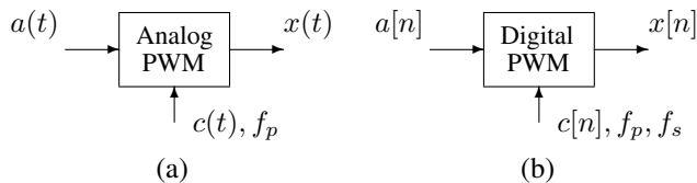
Fig. 2. Block diagram of (a) analog PWM and (b) digital PWM.
