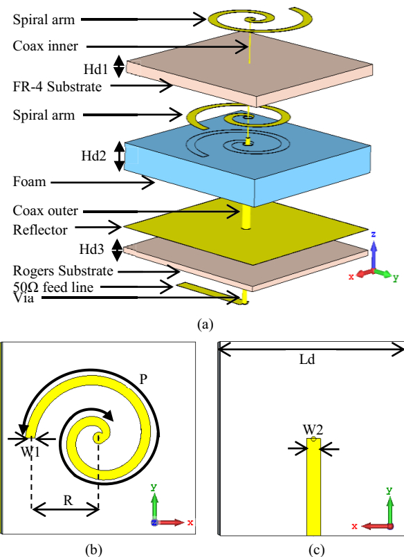
Fig. 1. The proposed antenna (a) exploded geometry (b) front view (c) rear view
